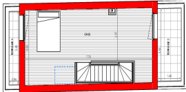
LOT 301 (BAT E) R+2 1:50
